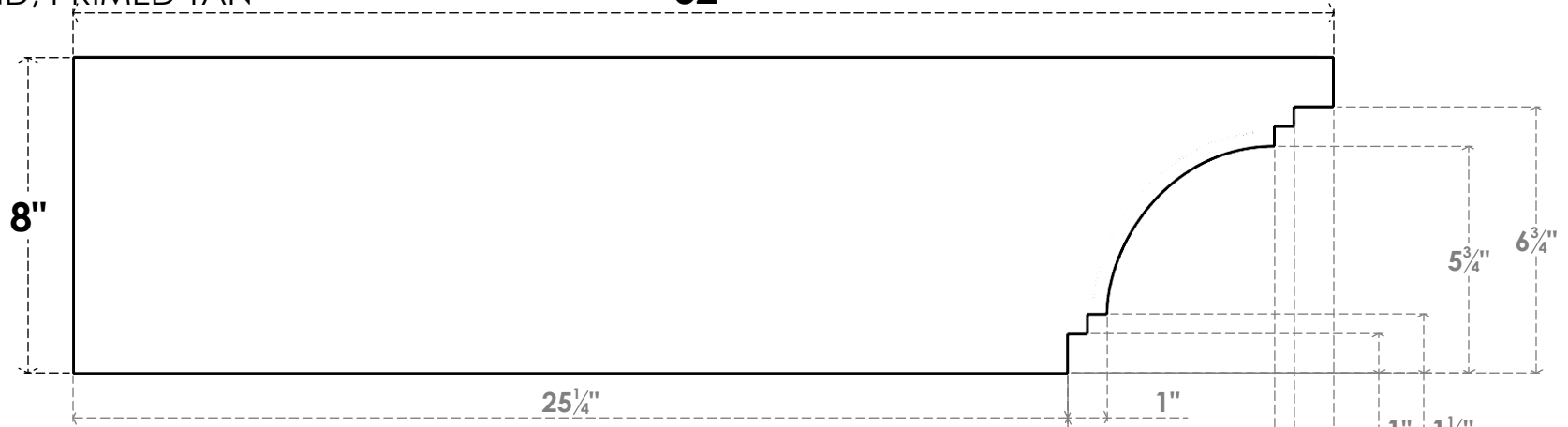
SIDE PROFILE
